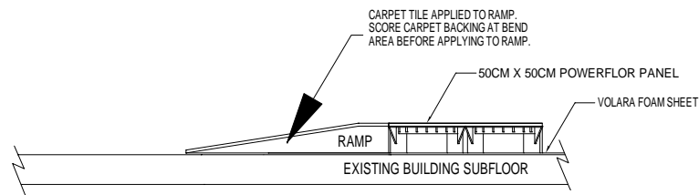
TYPICAL RAMP INSTALLATION
